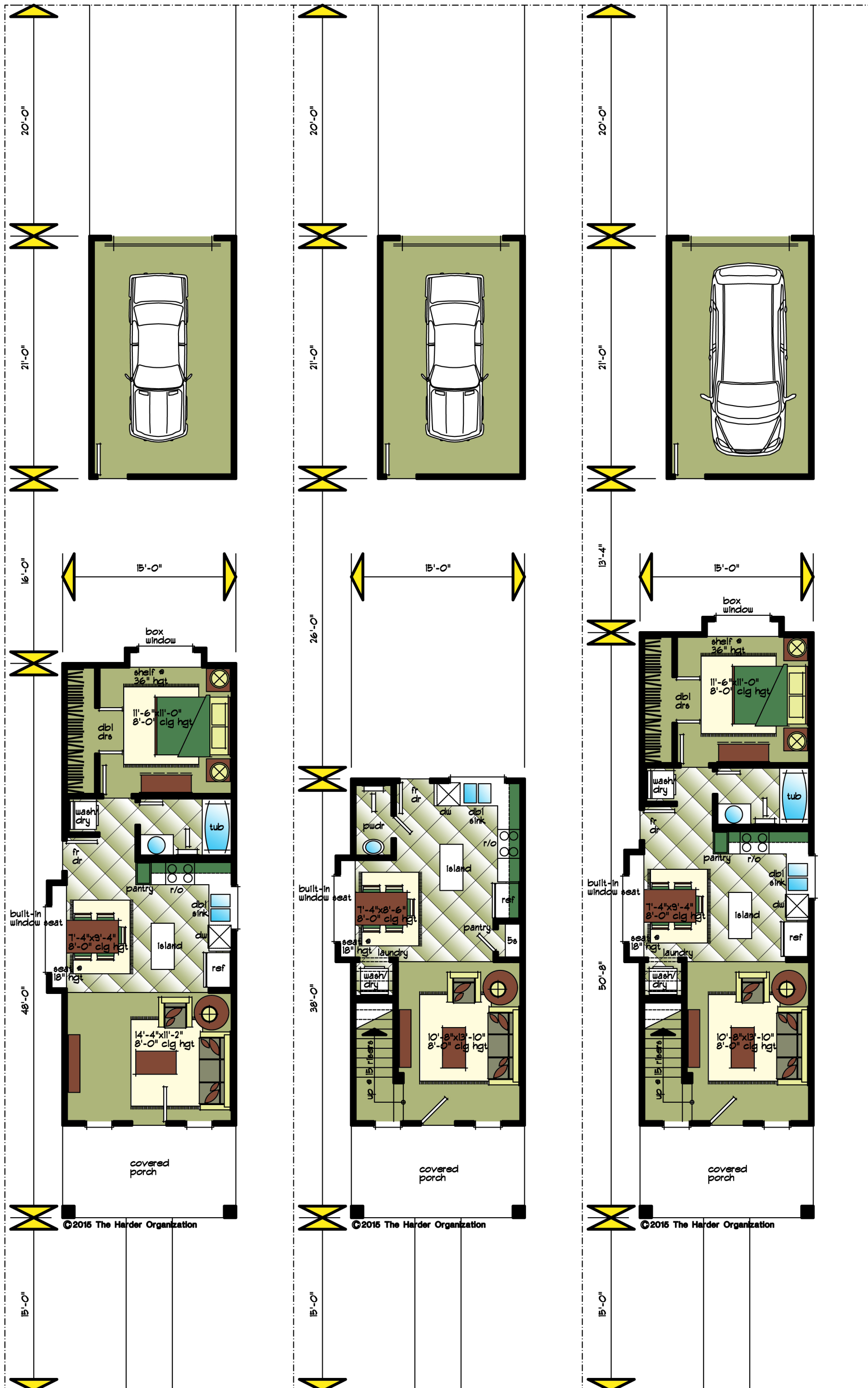
flr plan a standard 600 sq ft 1 st flr plan b standard 848 sq ft 1 st flr plan c standard 1058 sq ft
