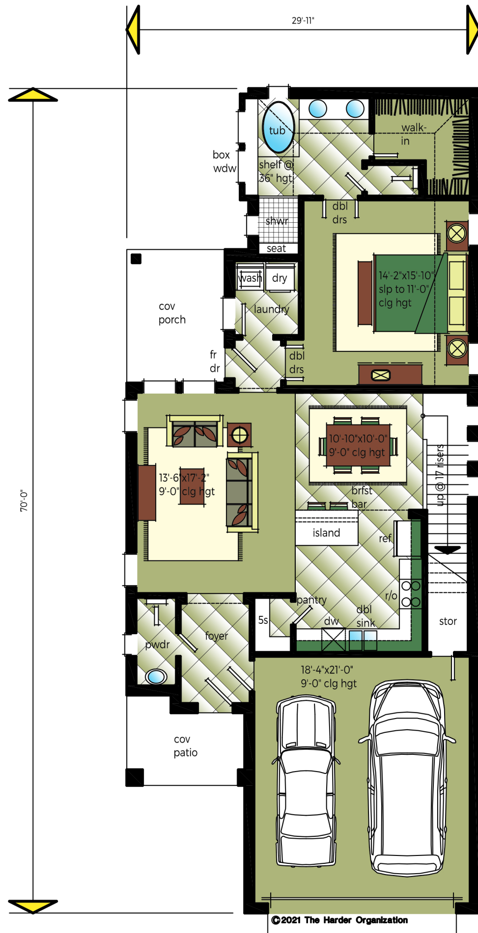
1st floor plan e
